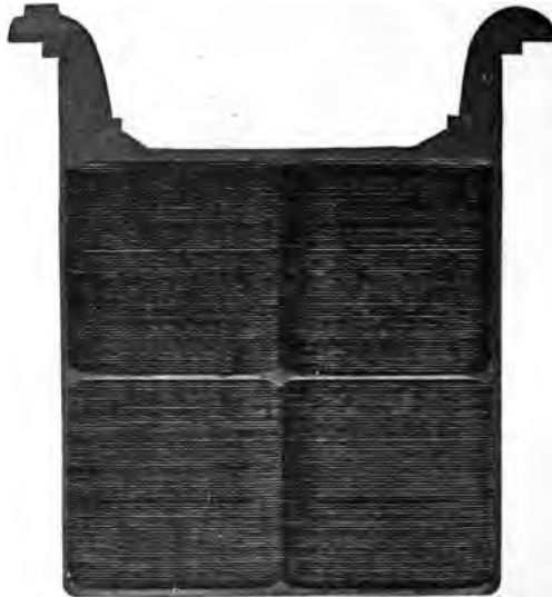
FIG. 314.—“Unformed” Plate of One Pattern of “Gould” Storage Cell. The particular plate shown has total outside dimensions of 6x6 inches. The clear outline of the grooves indicates absence of oxides, due to action of “forming” solutions, or charging current.
